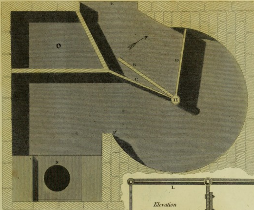
Plan
