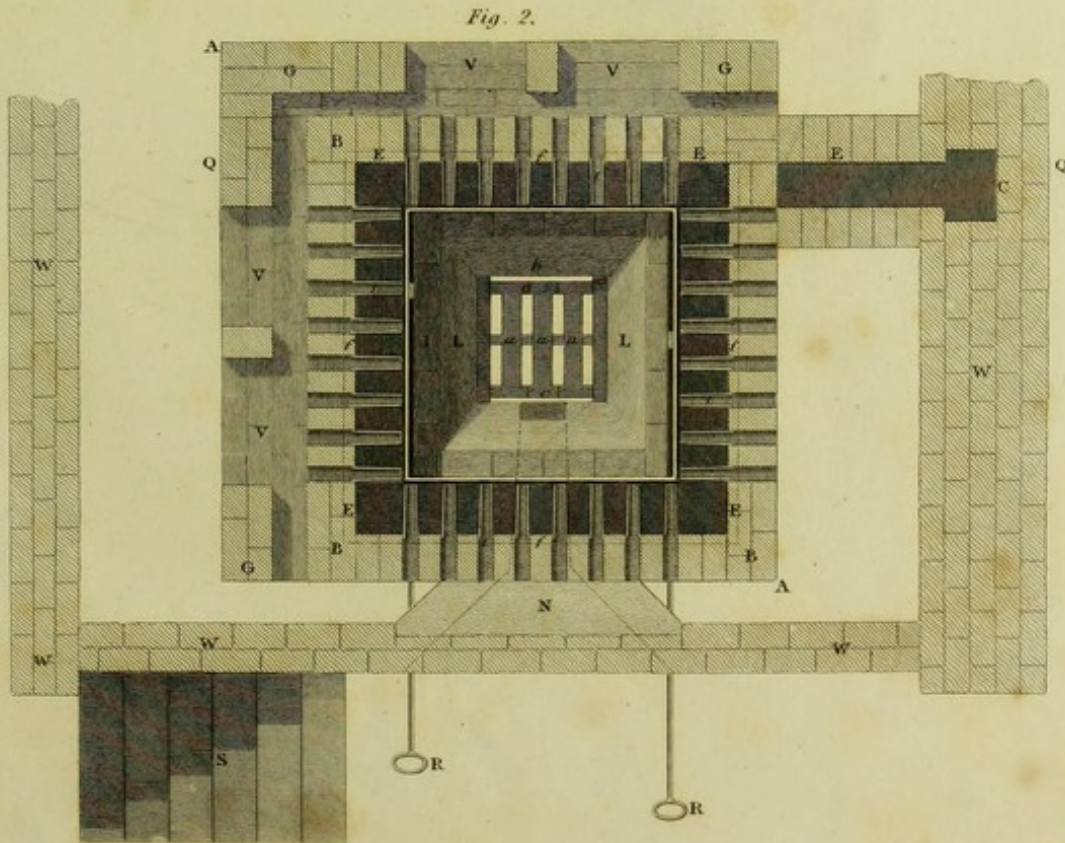
Plan of the Hot Air Stove.
